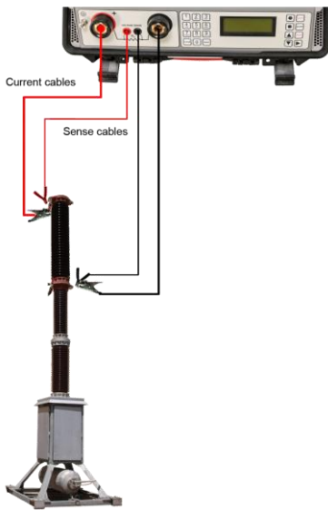
Micro Ohmmeter cable connection on live tank circuit breaker
