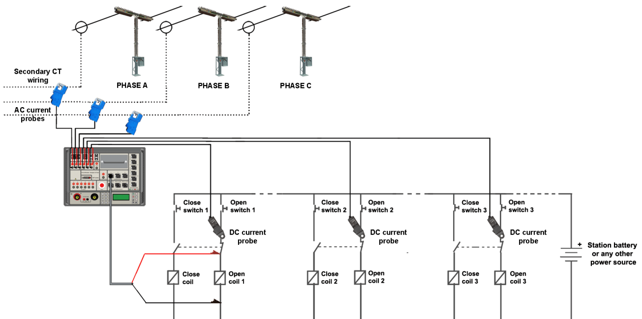
Connecting the current probes for measurement of the coil current and the line currents during the “First trip” test
