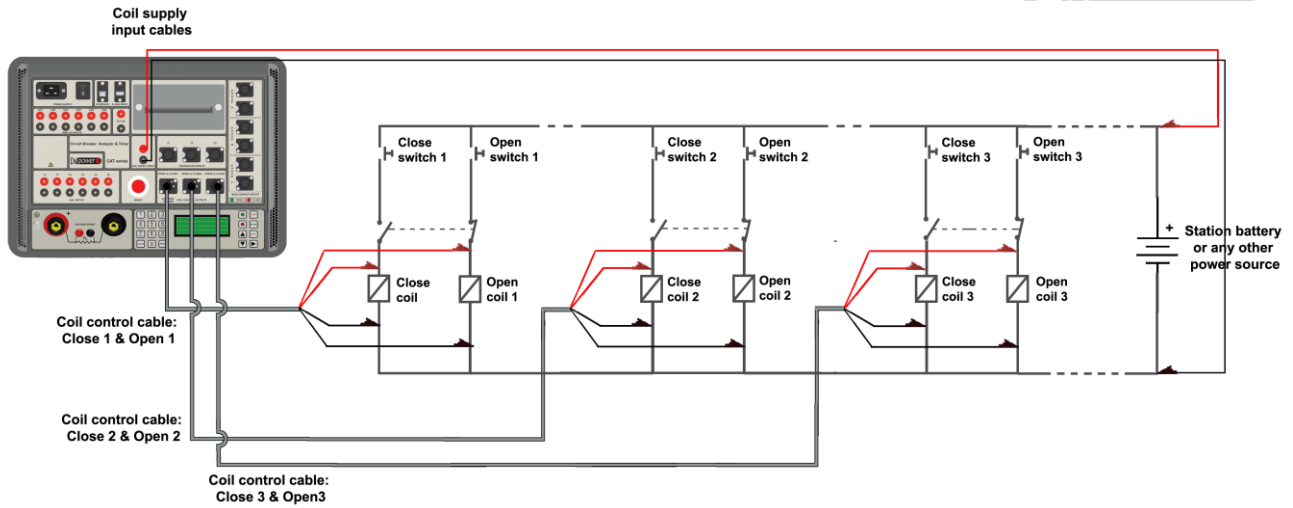
Connecting the coil control cables to open and close coils of the single pole circuit breaker
