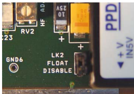
Figure 2-1. Float Enable/Disable Jumper
