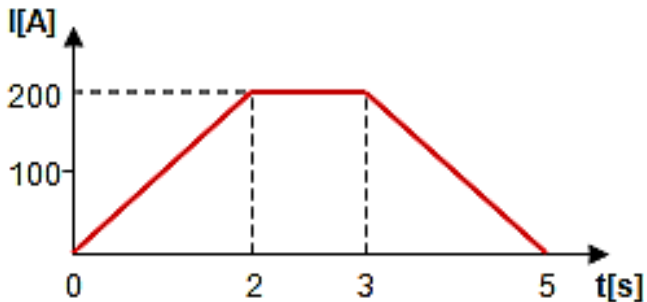
Figure 1 -Single test ramp
