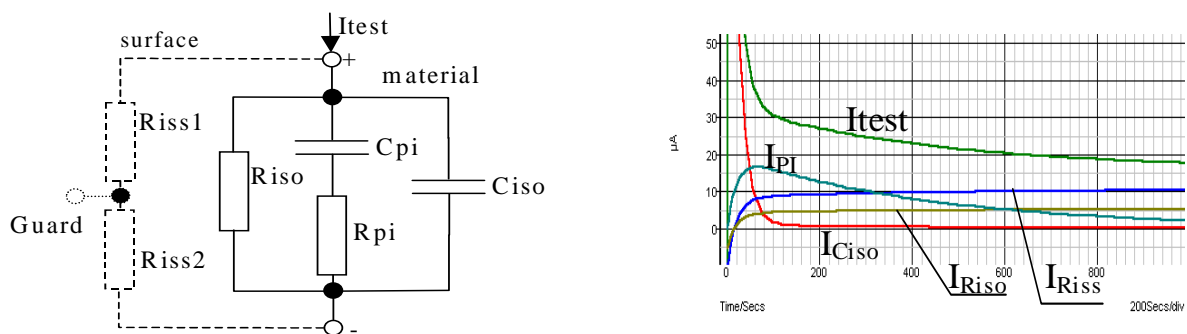
Figure 5.1: Insulating material
