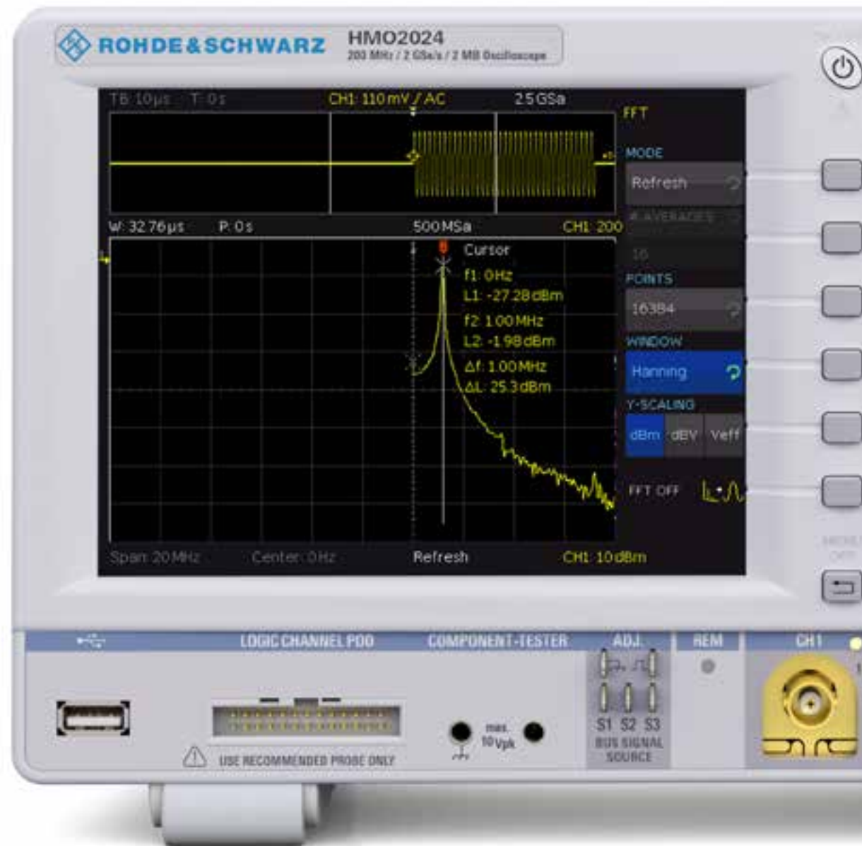
Figure 5: FFT analysis of a sine burst signal with Hanning window function
