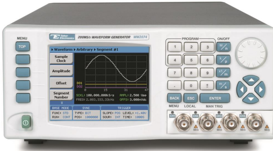
Figure 1-1, Model 2074
