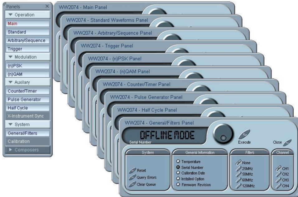
Figure 1-2, ArbConnection – The Control Panels
