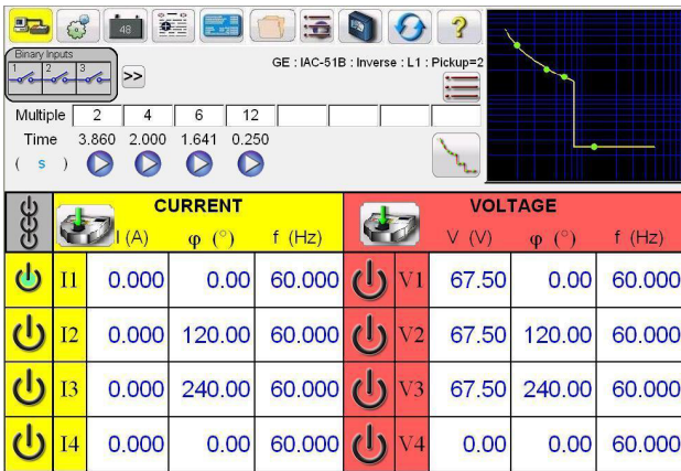
Figure 4 Timing G.E. IAC51B Overcurrent Relay (4 Channel unit shown)
