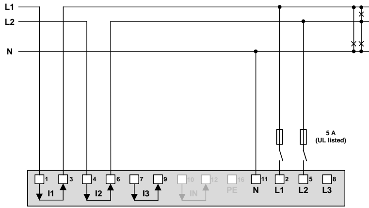
Direct connection
