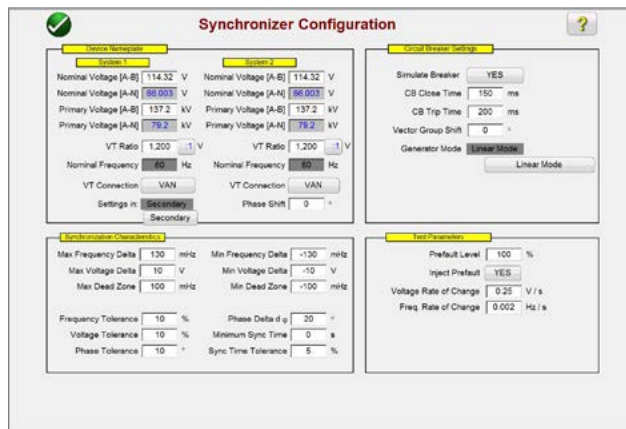
Synchronizing Configuration Screen
