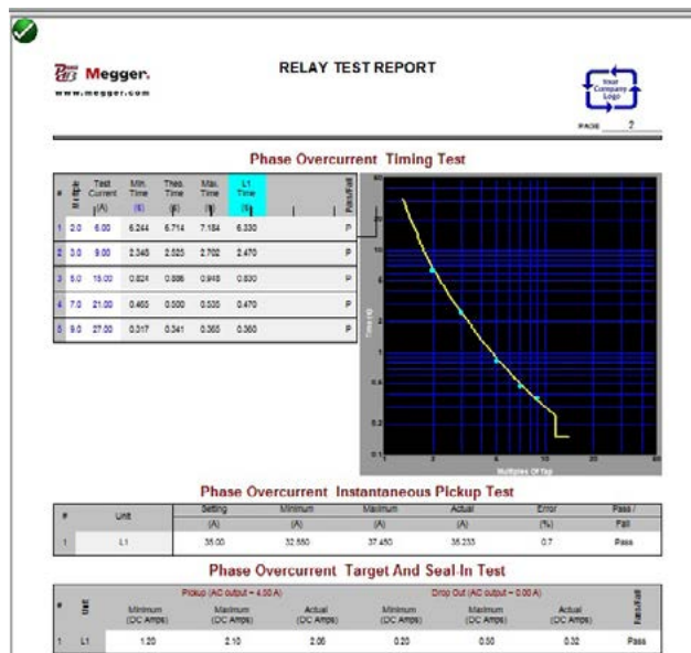
Timing Westinghouse CO-11 Overcurrent Relay
