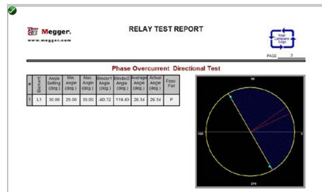
Page 2 Phase Directional Test Report
