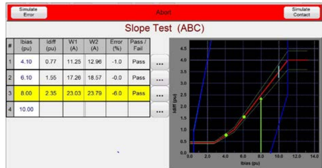
Transformer Differential Slope Test
