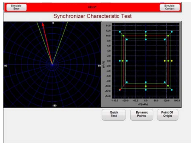
Dynamic Synchronizing Test Screen
