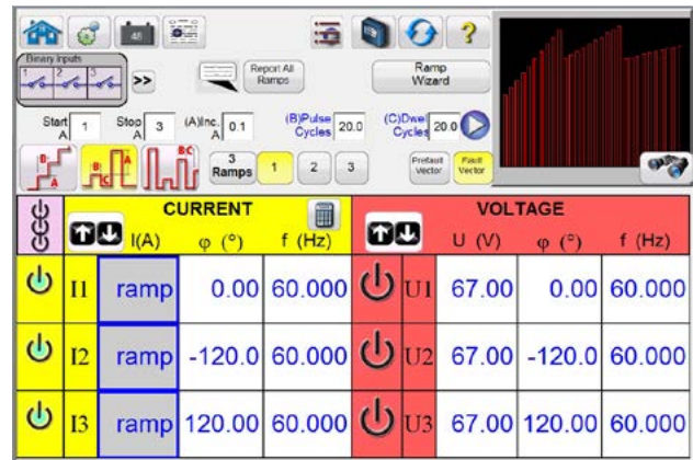
Three Phase Pulse Ramp
