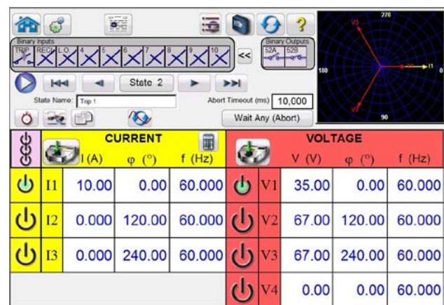
Multi-State Sequence Test Screen
