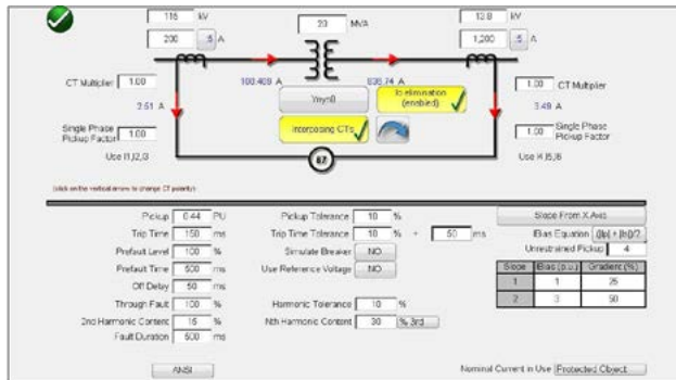
ANSI Transformer Differential Model
