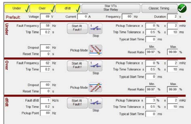
Frequency Relay Configuration Screen
