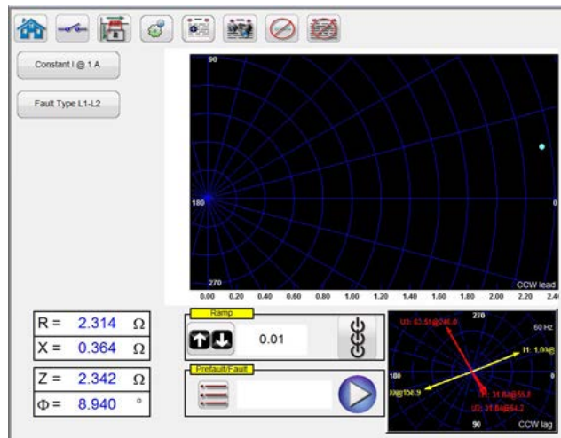
Easy Z Test Screen
