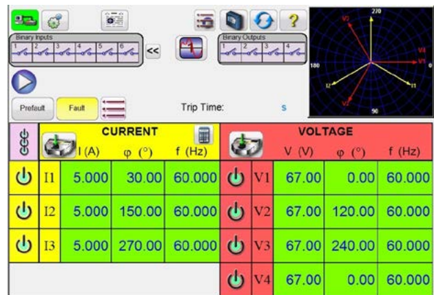
Manual User Interface 1 - Color Accents when Selected Outputs are on
