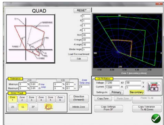
Generic QUAD Setting Screen
