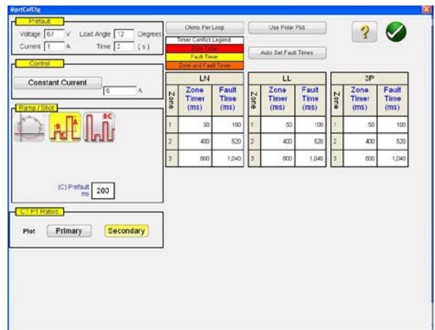
Generic QUAD Test Setup Screen
