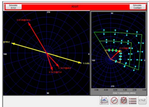
Generic QUAD Real-Time Test Screen
