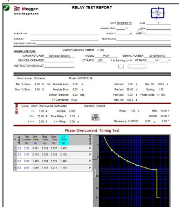
Test Report MiCOM P124 Timing Test Report
