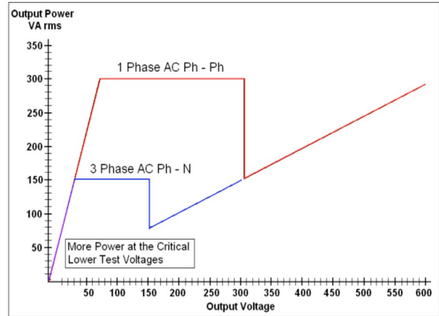
"PowerV" Voltage Amplifier Output Power Curves
