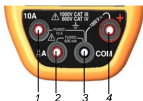
Figure 4 : the terminals
