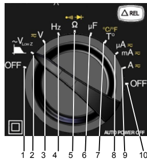
Figure 1 : the switch
