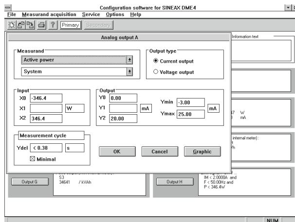
Fig. 11. Programming of the output quantities.
