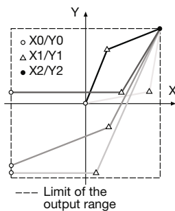
Fig. 9. Examples of settings with bent characteristic.
