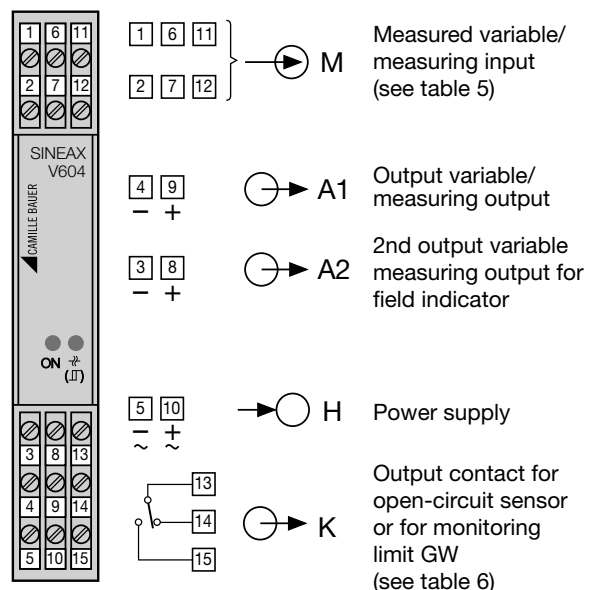
Fig. 9. Terminal allocation.
