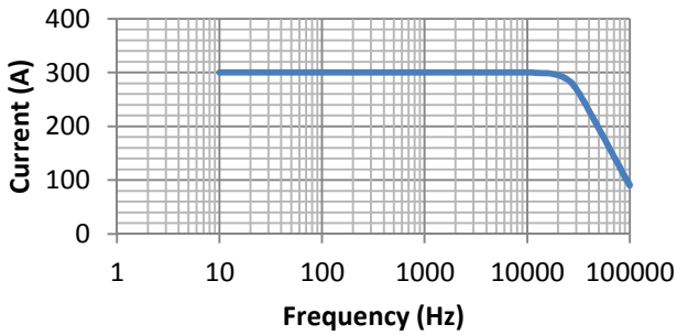
Metraflex 300M I * f De-rating curve
