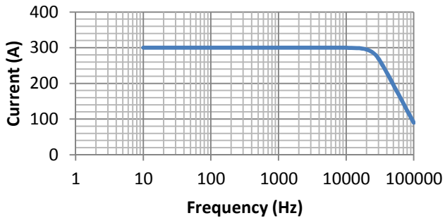
Metraflex 300M I * f De-rating curve
