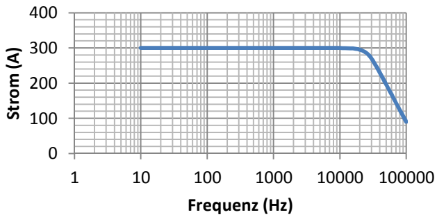
Metraflex 300M I * f Derating-Kurve
