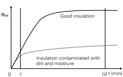
Time diagrams of good and bad insulation tested with the time-rise method
