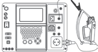
Insulation resistance test for Class II device
