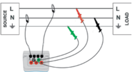
Connection to 1-phase 3-wire system
