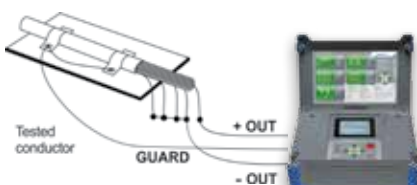
Measurement of insulation resistance of communication cable using the guard terminal. Resistance is measured between one lead and other leads
