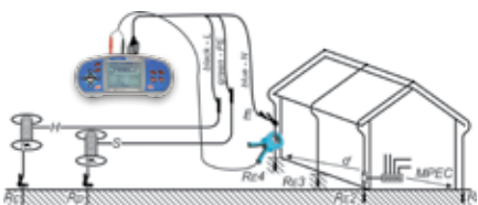
Circuit for one clamp measurement
