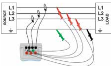
Connection to 3-phase 3-wire system
