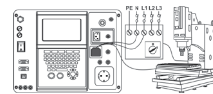
Loop impedance test
