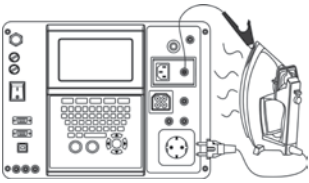
Touch leakage current test for Class II device
