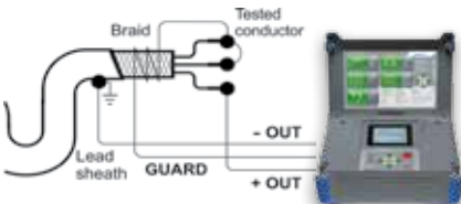
Measurement of insulation resistance of a cable between a conductor and lead sheath
