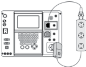
Active polarity test
