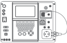
Polarity test
