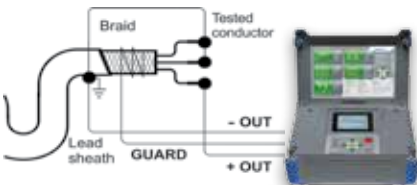
Measurement of insulation resistance of cable between one conductor against other conductors and lead sheath using the guard terminal to avoid leakage effects at the end of cable
