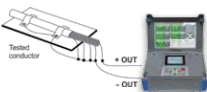
Measurement of insulation resistance between one lead of communication cable against other leads and sheath
