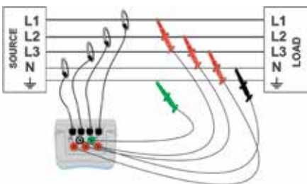
Connection to 3-phase 4-wire system
