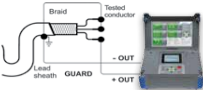
Measurement of insulation resistance of cable between one conductor against other conductors including lead sheath
