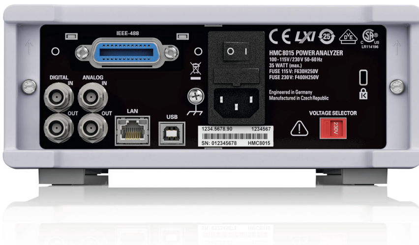
Rear panel interfaces (shown here: R&S®HMC8015-G with GPIB interface).
